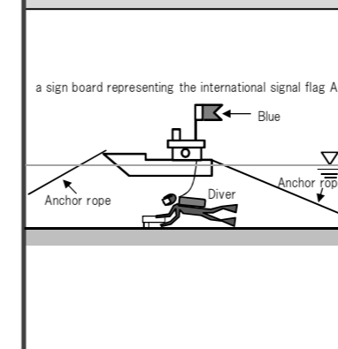
Fig.-2 Shape of diver's boat
