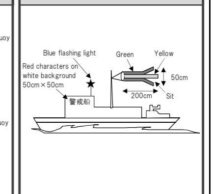
Fig.-4 Shape of Patrol boat
