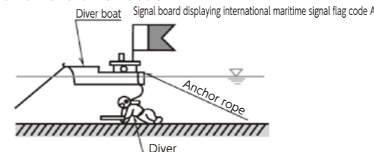
Figure 5: Signal on the diver boat
