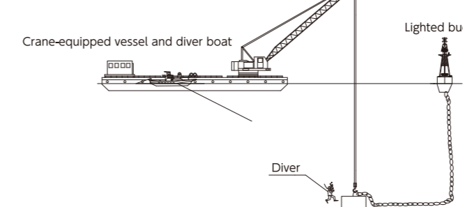
Figure 3: Lighted buoy relocation and restoration plan
