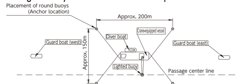
Figure 3: Lighted buoy relocation and restoration plan
