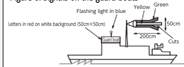
Figure 6: Signals on the guard boats
